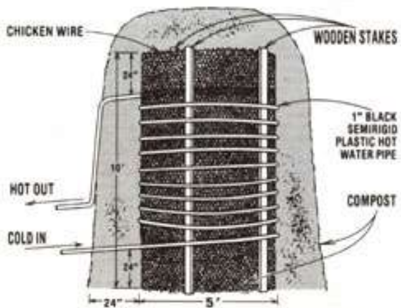
CROSS SECTION OF JEAN PAIN'S COMPOST WATER HEATER
